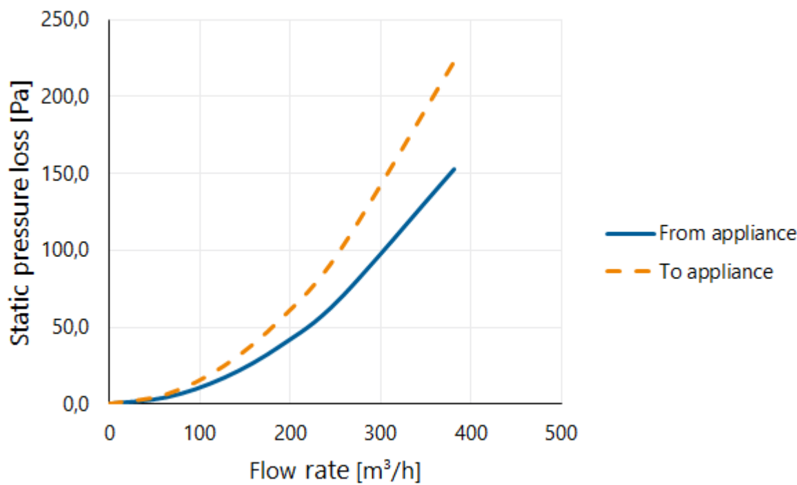
Pressure loss
