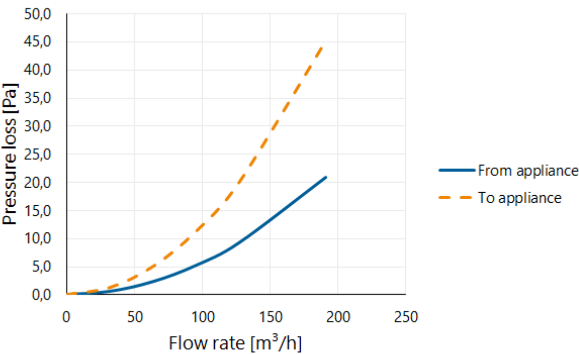
Pressure loss
